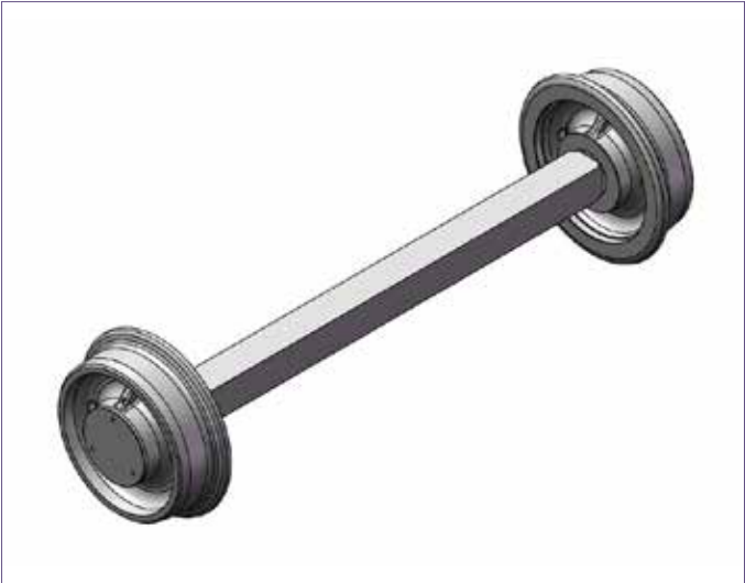
Essieu roue 400MT 15T - Montage 412 Axle wheel 400MT, load 15T - Mounting 412
