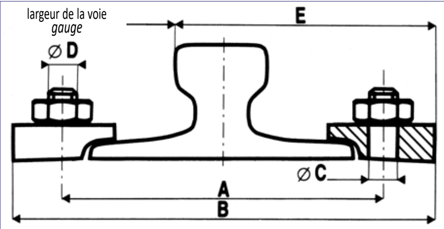
Rail pont roulant Crane rail
