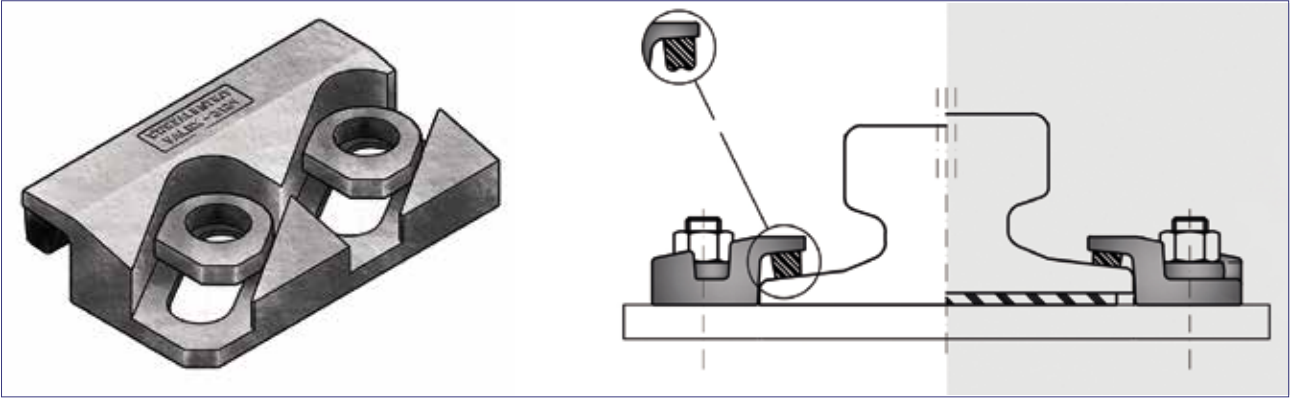
Fixation indirecte (clip à boulonner) Indirect fastening system (boltable)
