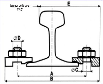
Rail vignole Vignole rail
