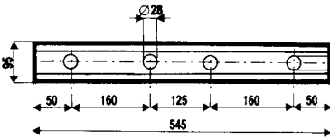
ECLISSE / FISHPLATE
